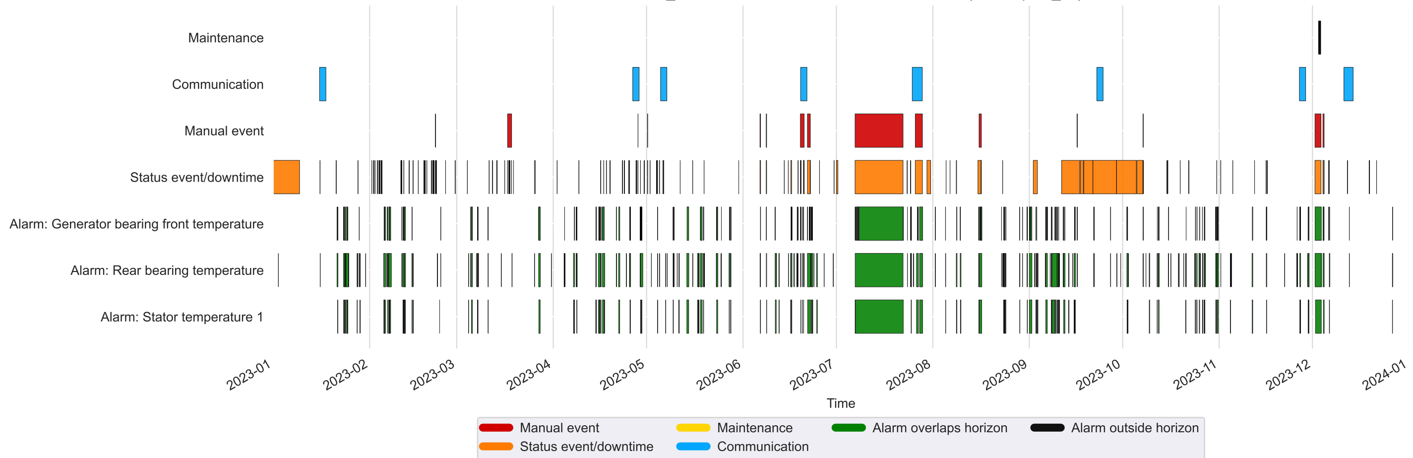
Kelmarsh_5: labelled intervals and detection alarms (2023, q950_c6)
