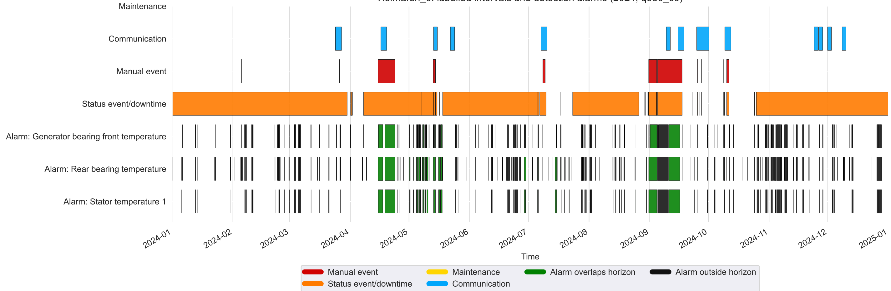
Kelmarsh_6: labelled intervals and detection alarms (2024, q950_c6)
