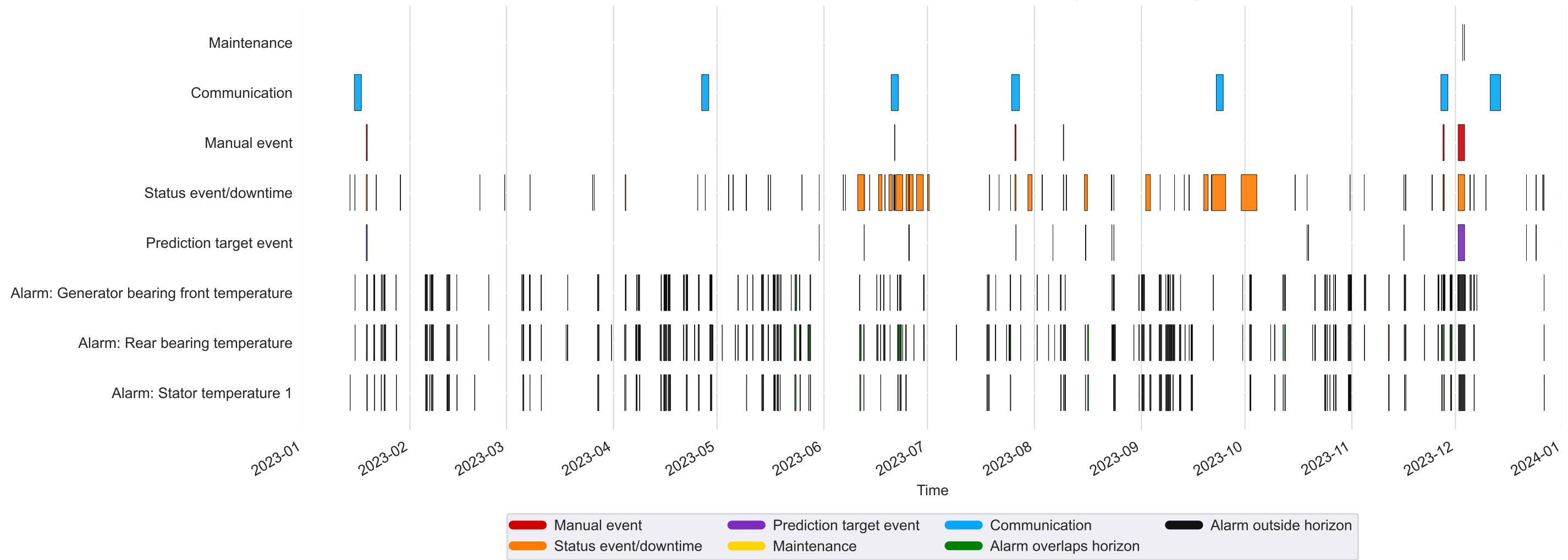
Kelmarsh_1: labelled intervals and detection alarms (2023, q950_c6)
