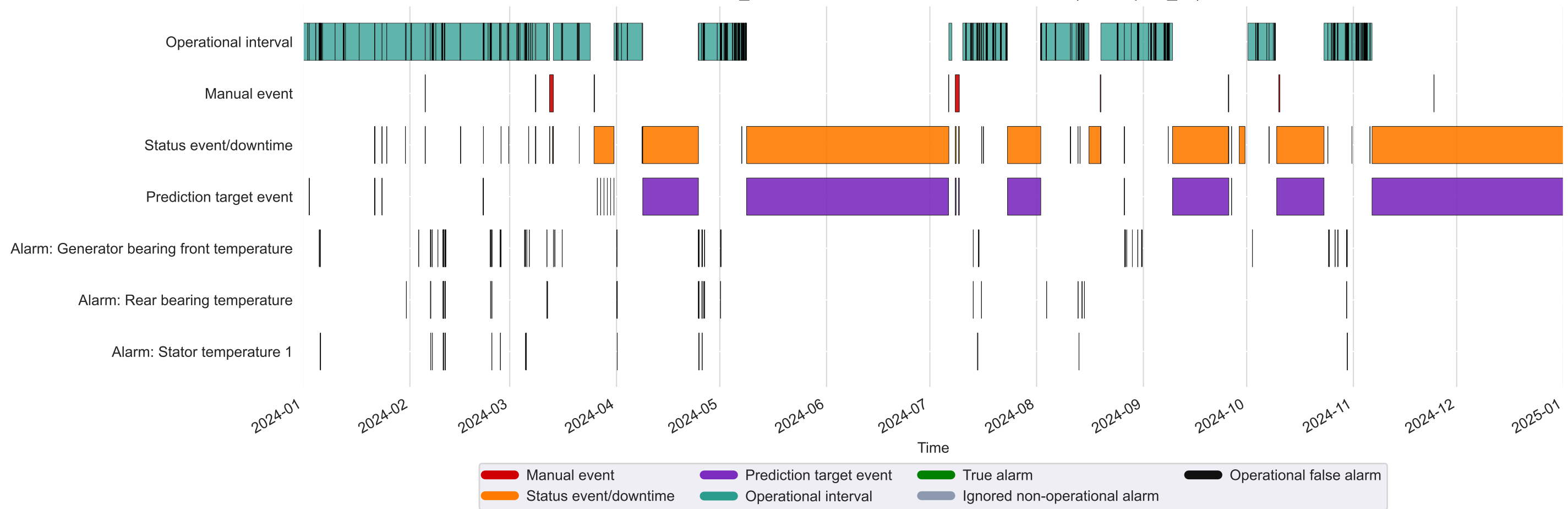
Kelmarsh_1: labelled intervals and detection alarms (2024, q950_c6)
