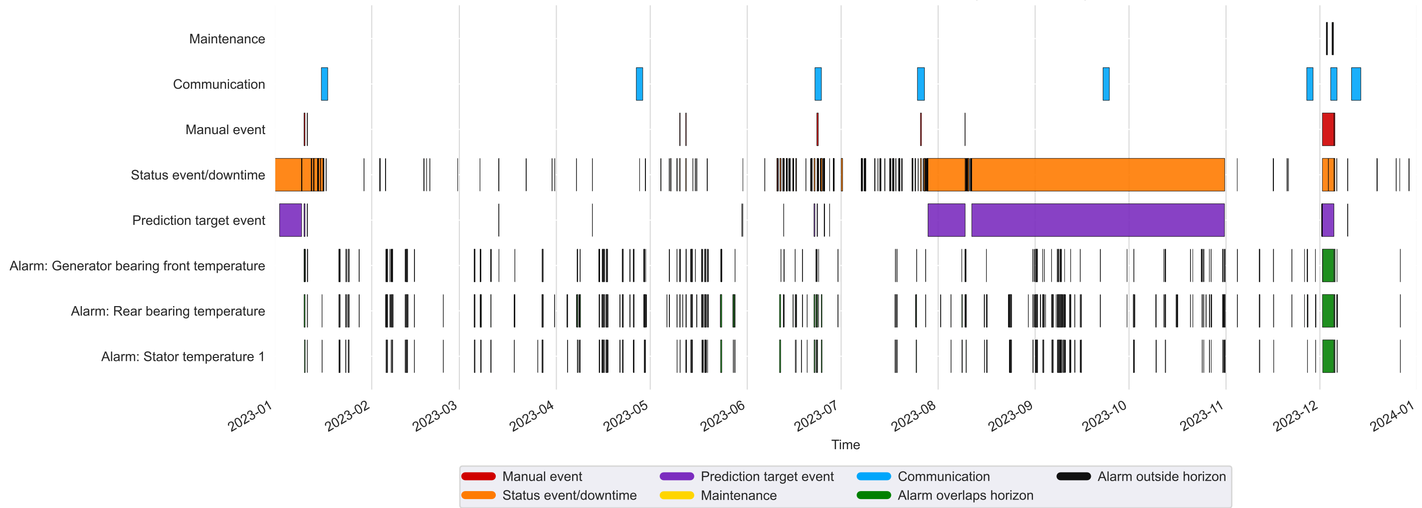
Kelmarsh_2: labelled intervals and detection alarms (2023, q950_c6)
