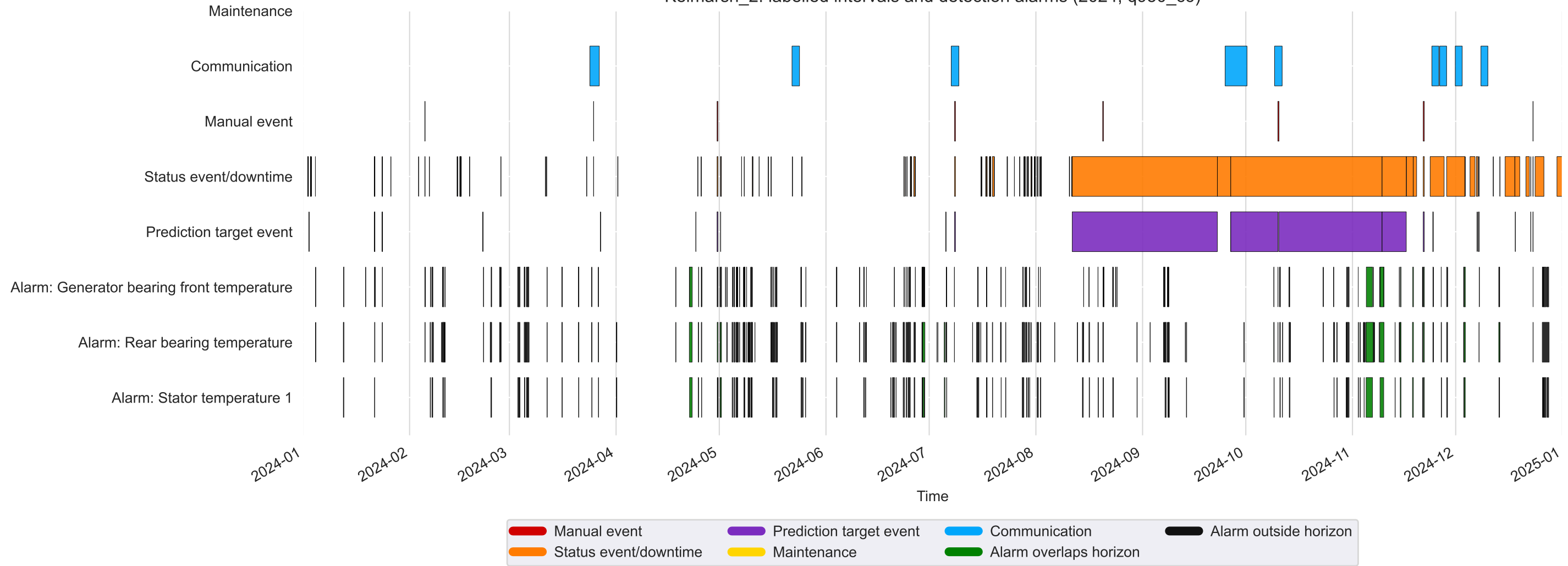
Kelmarsh_2: labelled intervals and detection alarms (2024, q950_c6)
