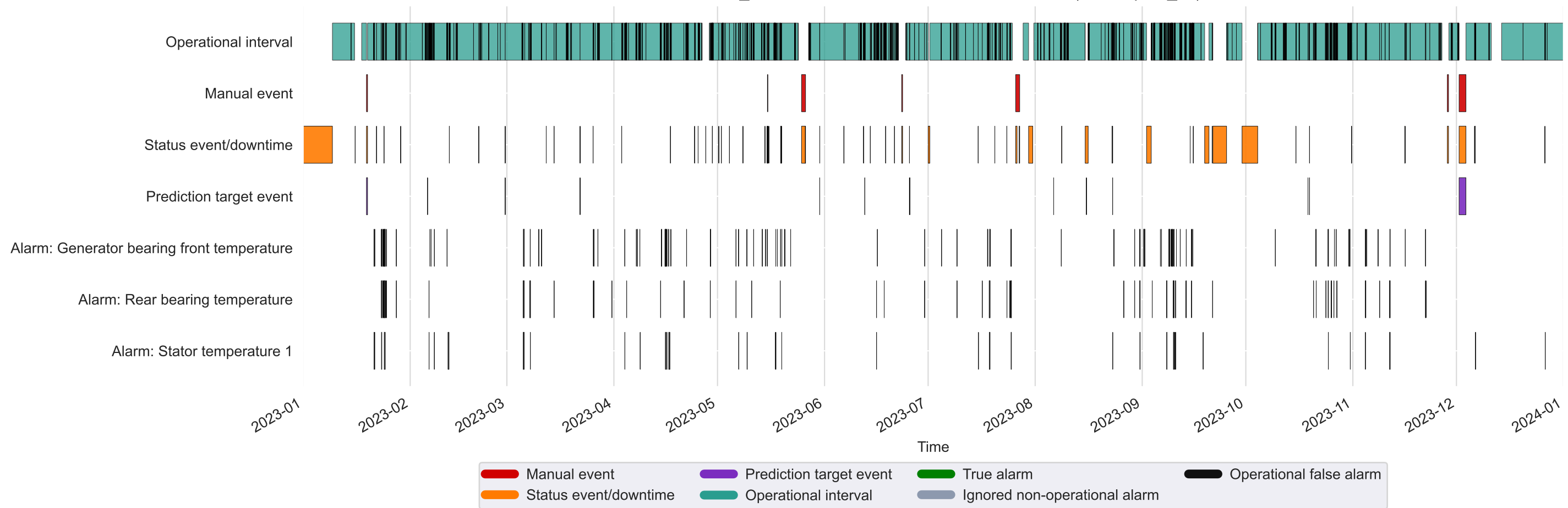
Kelmarsh_3: labelled intervals and detection alarms (2023, q950_c6)
