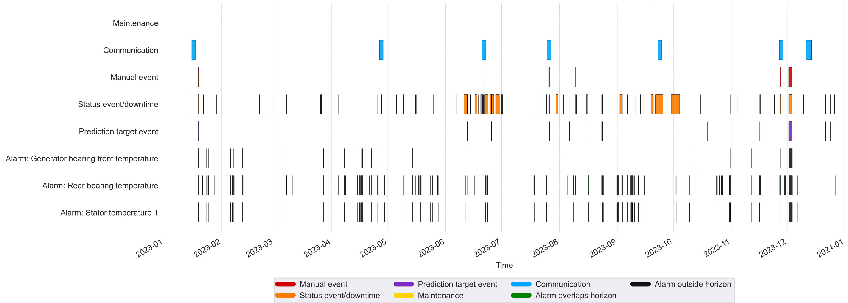
Kelmarsh_1: labelled intervals and detection alarms (2023, q990_c12)
