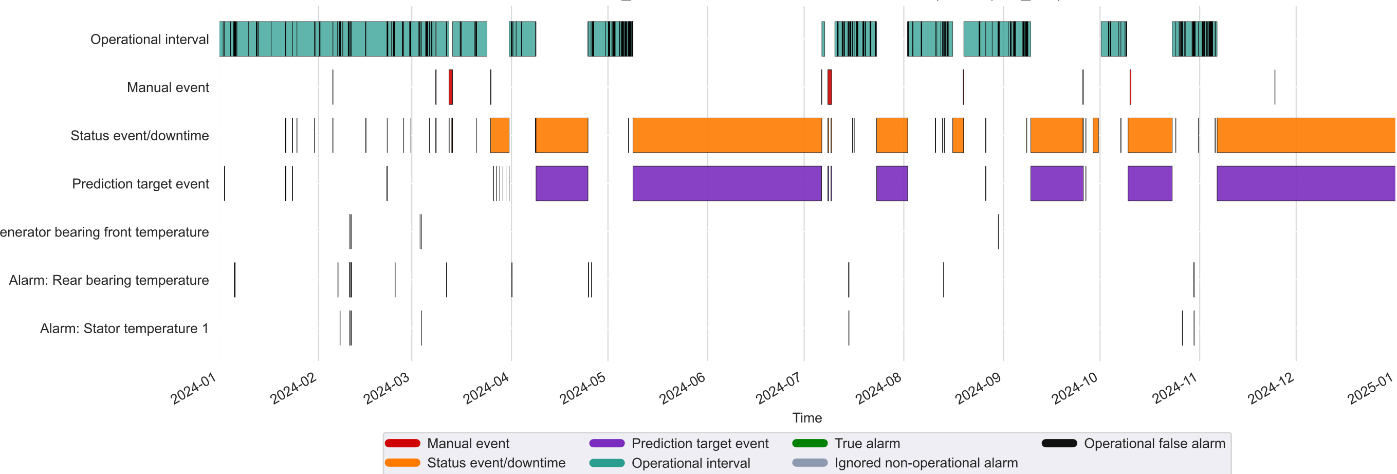
Kelmarsh_1: labelled intervals and detection alarms (2024, q990_c12)
