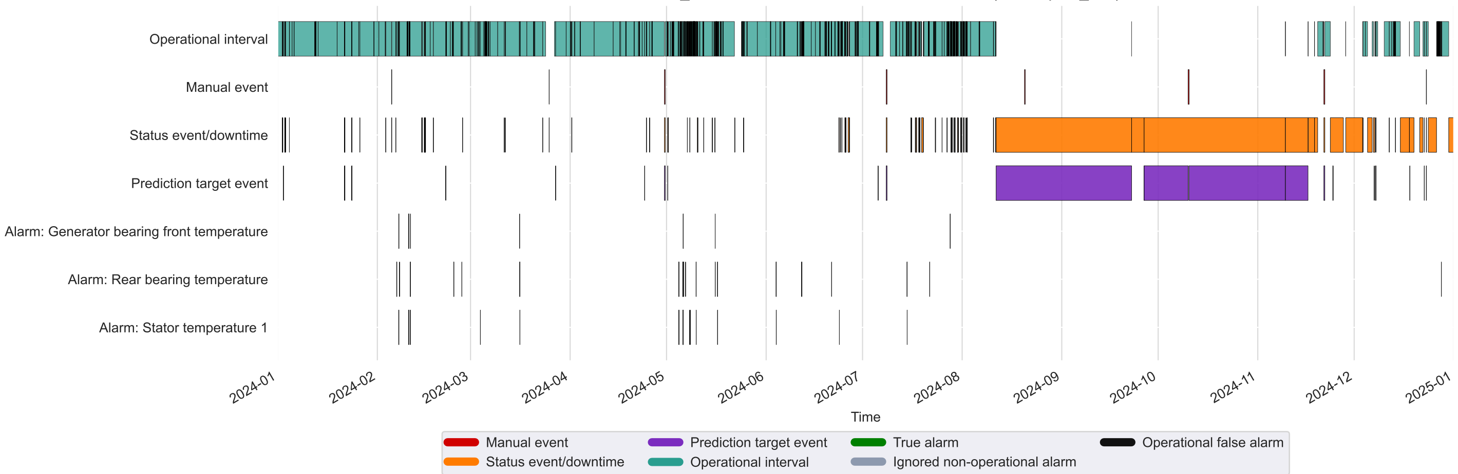
Kelmarsh_2: labelled intervals and detection alarms (2024, q990_c12)
