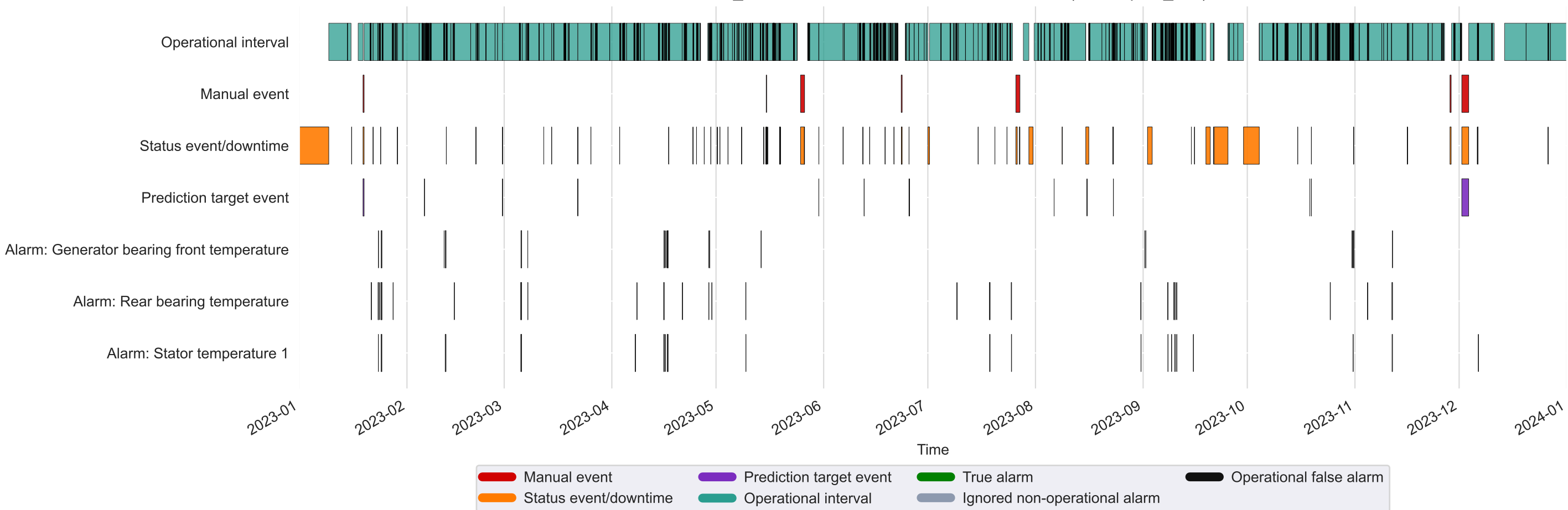
Kelmarsh_3: labelled intervals and detection alarms (2023, q990_c12)
