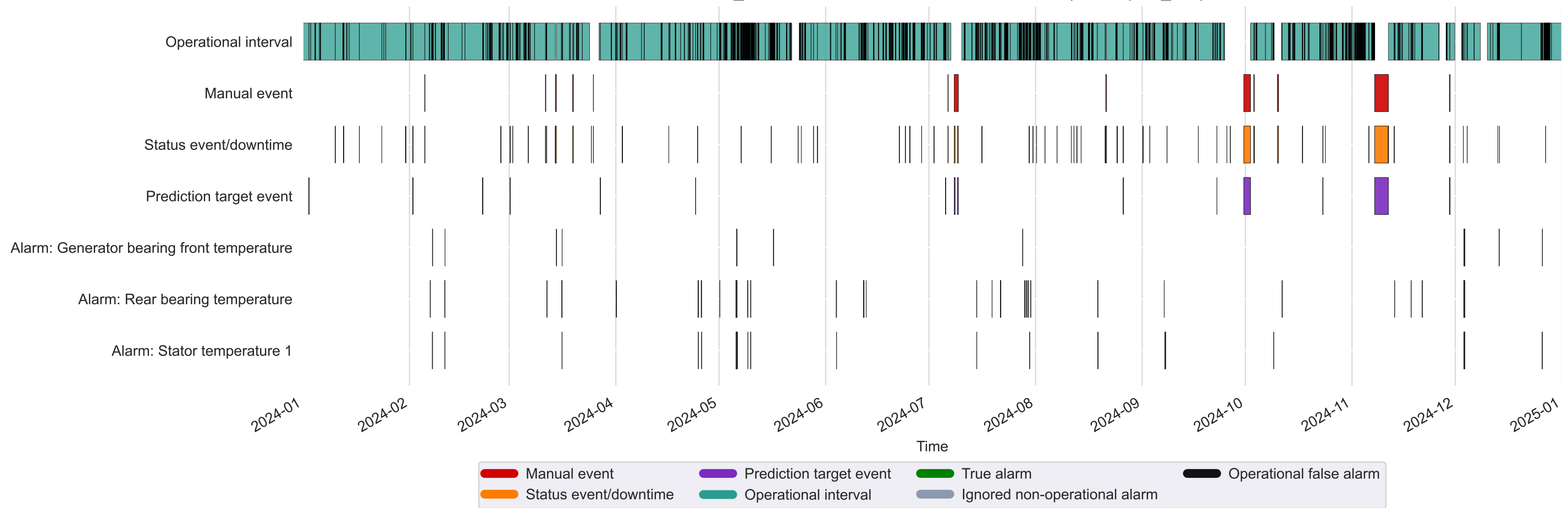
Kelmarsh_3: labelled intervals and detection alarms (2024, q990_c12)
