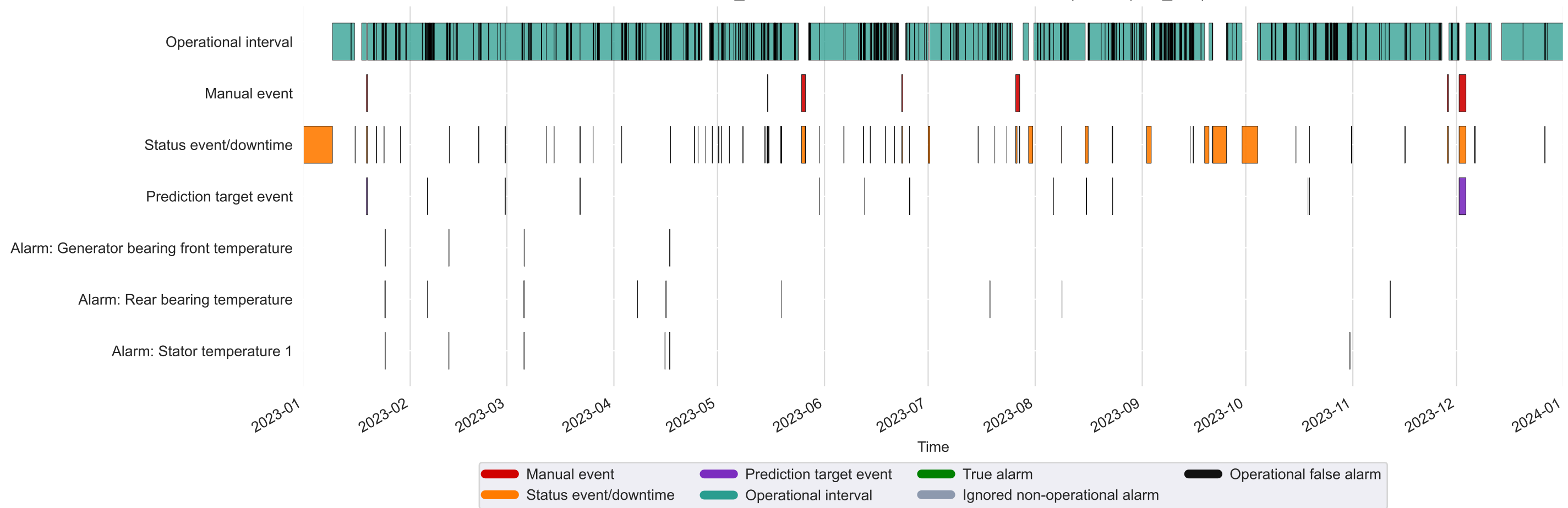
Kelmarsh_3: labelled intervals and detection alarms (2023, q990_c36)
