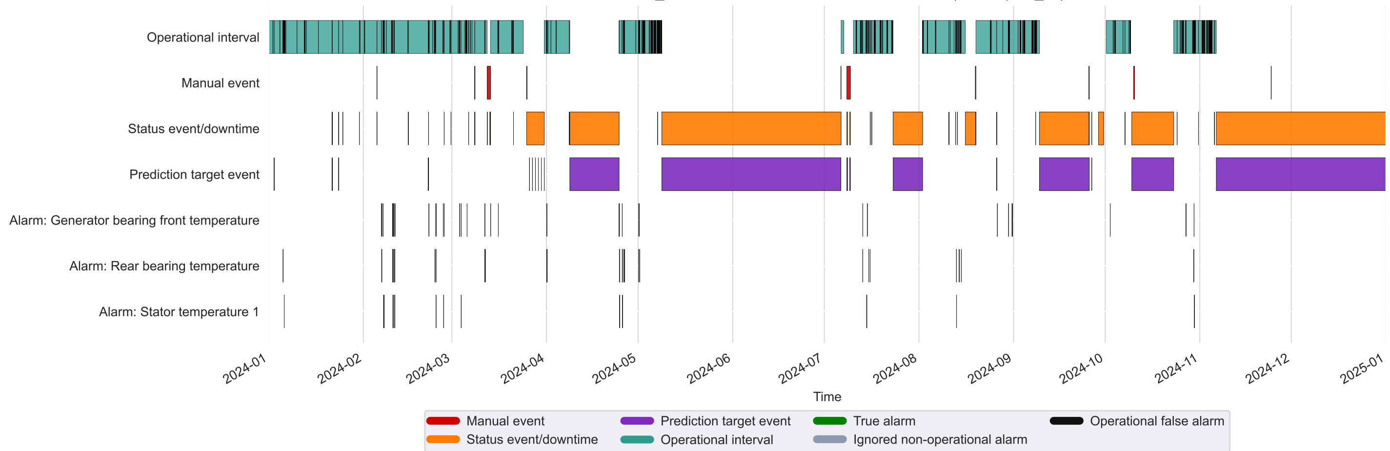
Kelmarsh_1: labelled intervals and detection alarms (2024, q990_c6)
