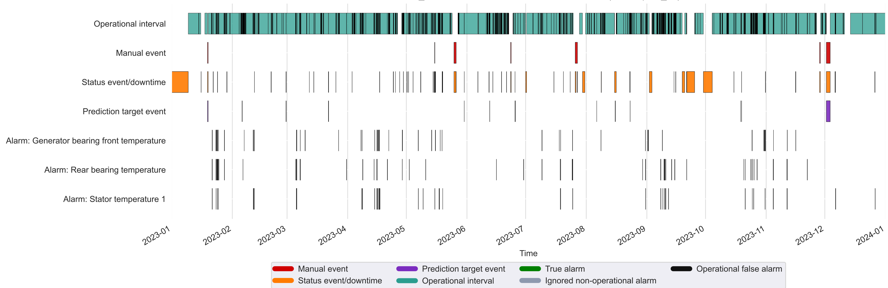
Kelmarsh_3: labelled intervals and detection alarms (2023, q990_c6)
