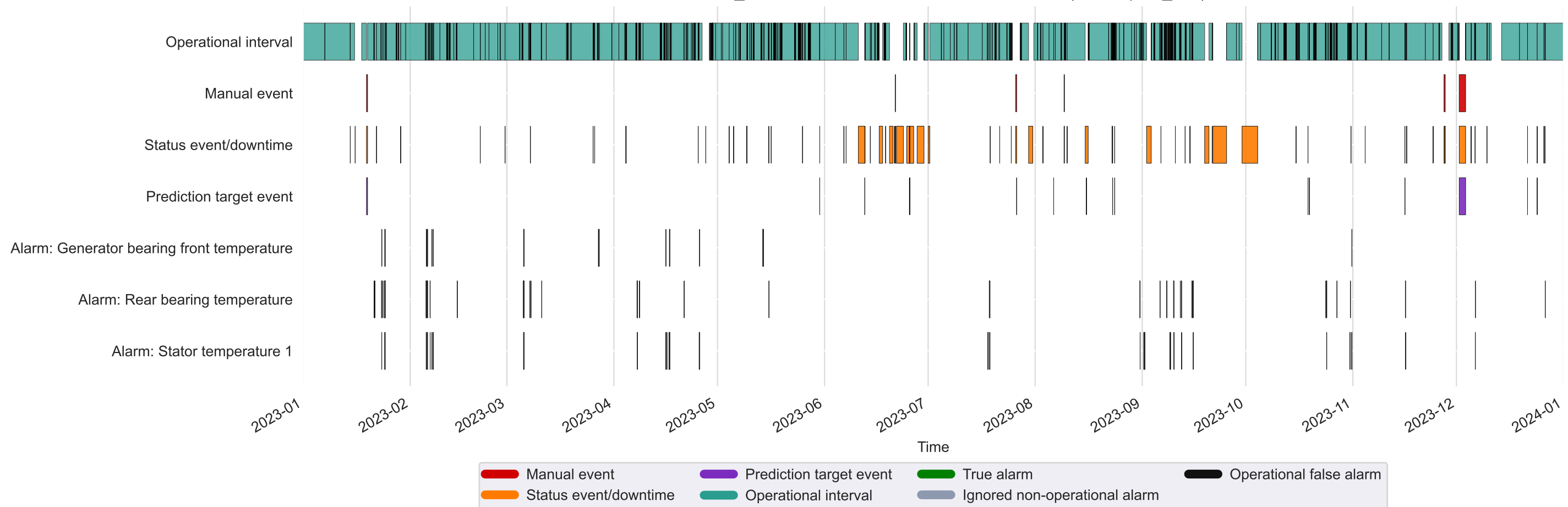
Kelmarsh_1: labelled intervals and detection alarms (2023, q995_c12)
