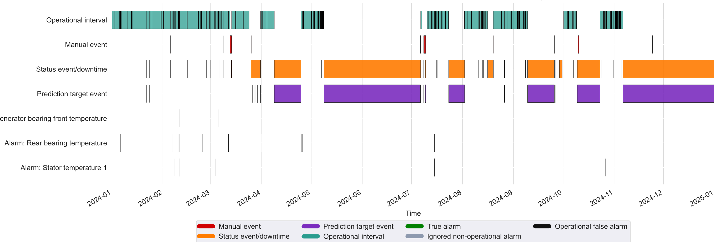
Kelmarsh_1: labelled intervals and detection alarms (2024, q995_c12)
