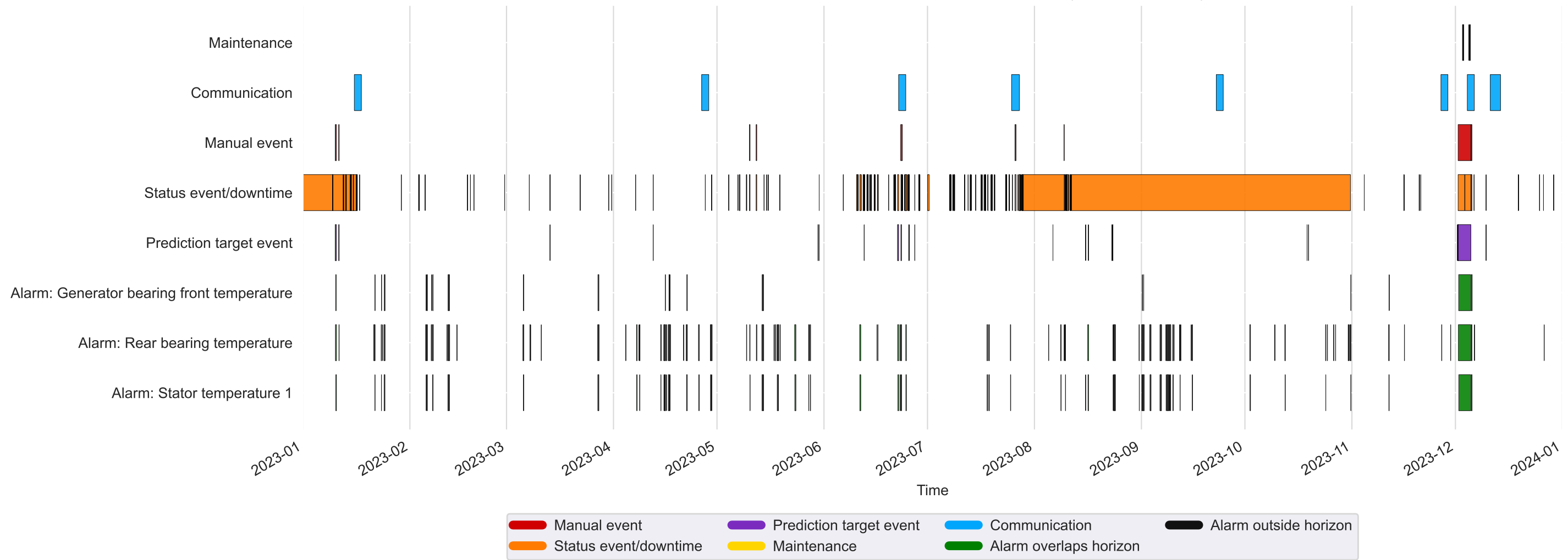
Kelmarsh_2: labelled intervals and detection alarms (2023, q995_c12)
