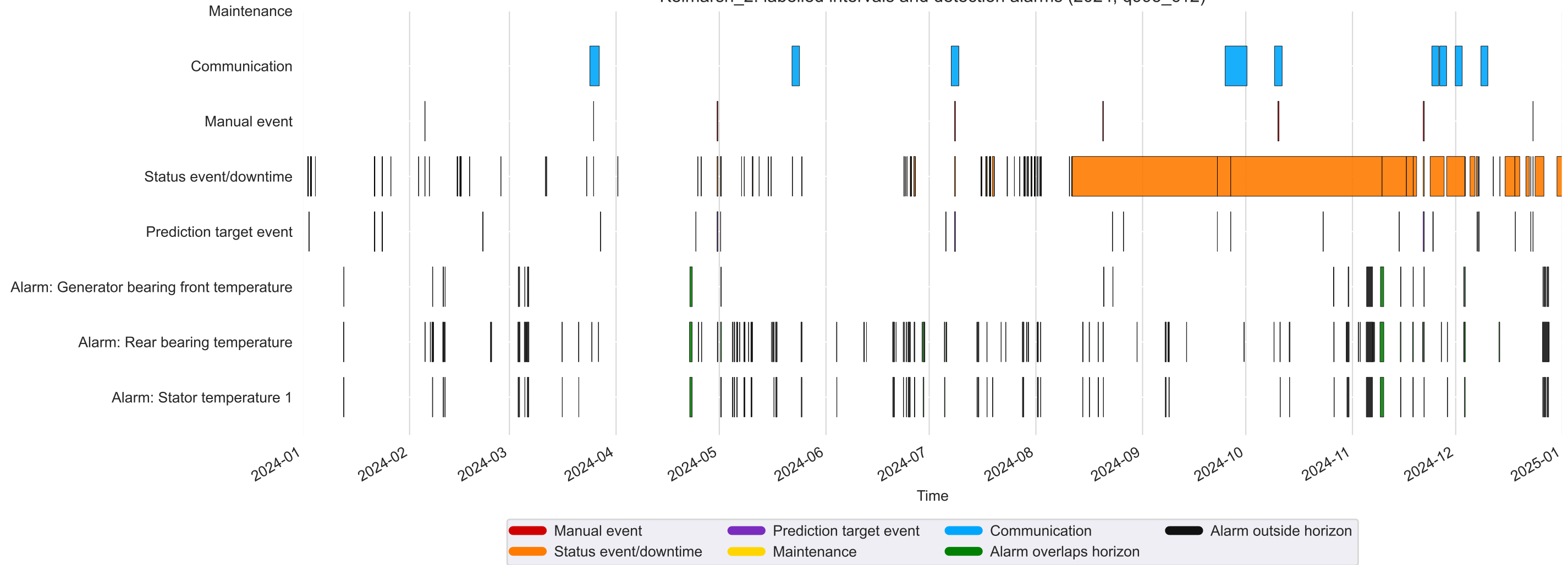
Kelmarsh_2: labelled intervals and detection alarms (2024, q995_c12)
