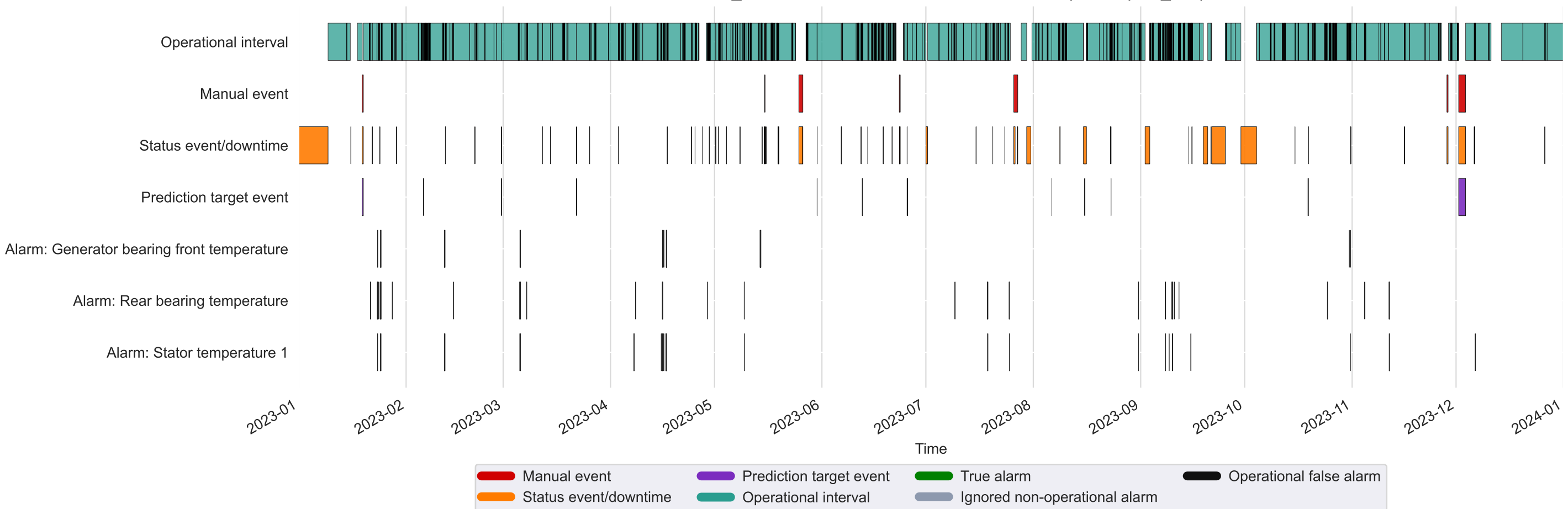
Kelmarsh_3: labelled intervals and detection alarms (2023, q995_c12)
