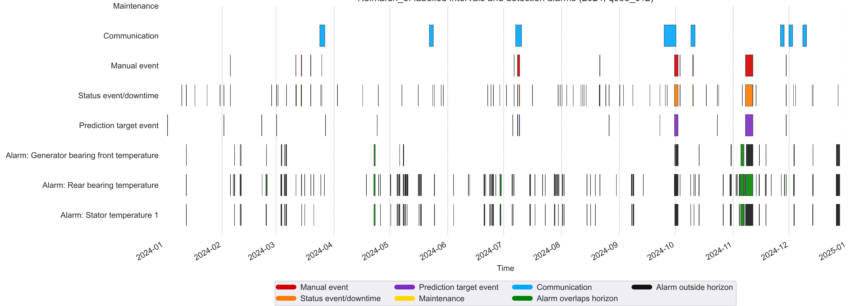
Kelmarsh_3: labelled intervals and detection alarms (2024, q995_c12)
