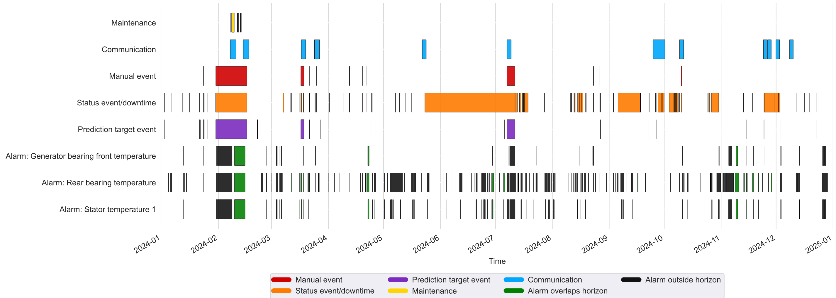
Kelmarsh_4: labelled intervals and detection alarms (2024, q995_c12)
