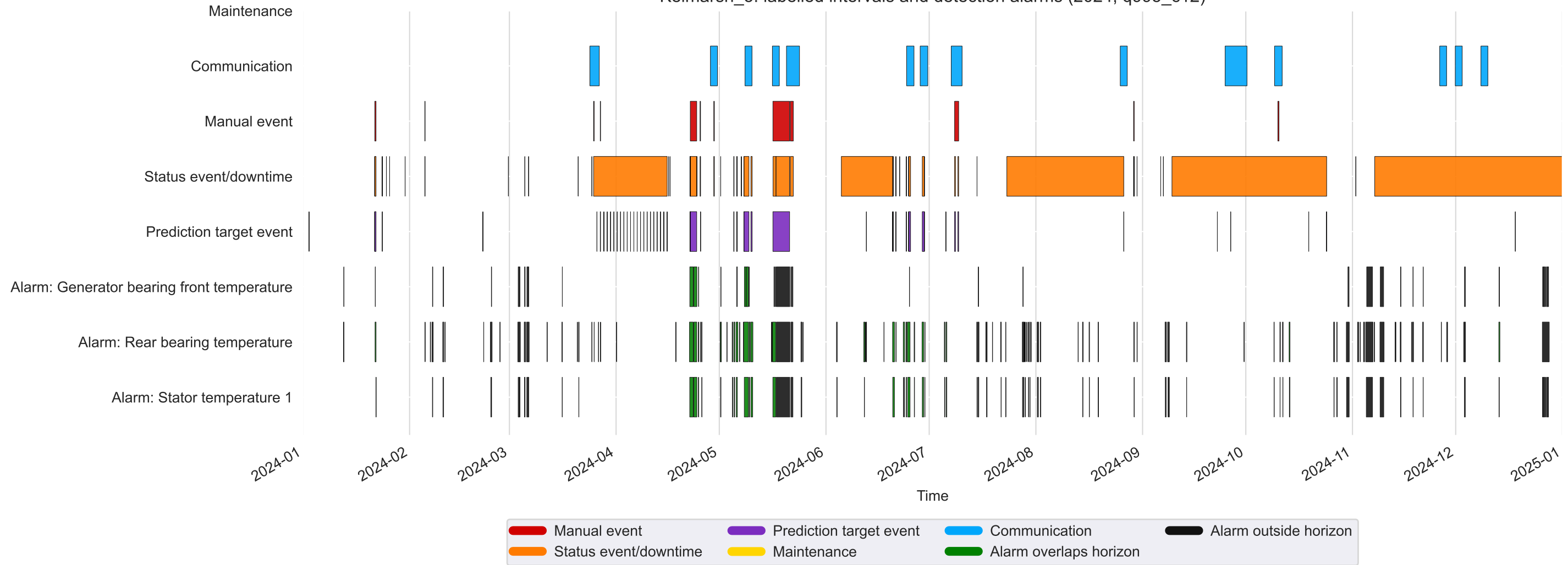
Kelmarsh_5: labelled intervals and detection alarms (2024, q995_c12)
