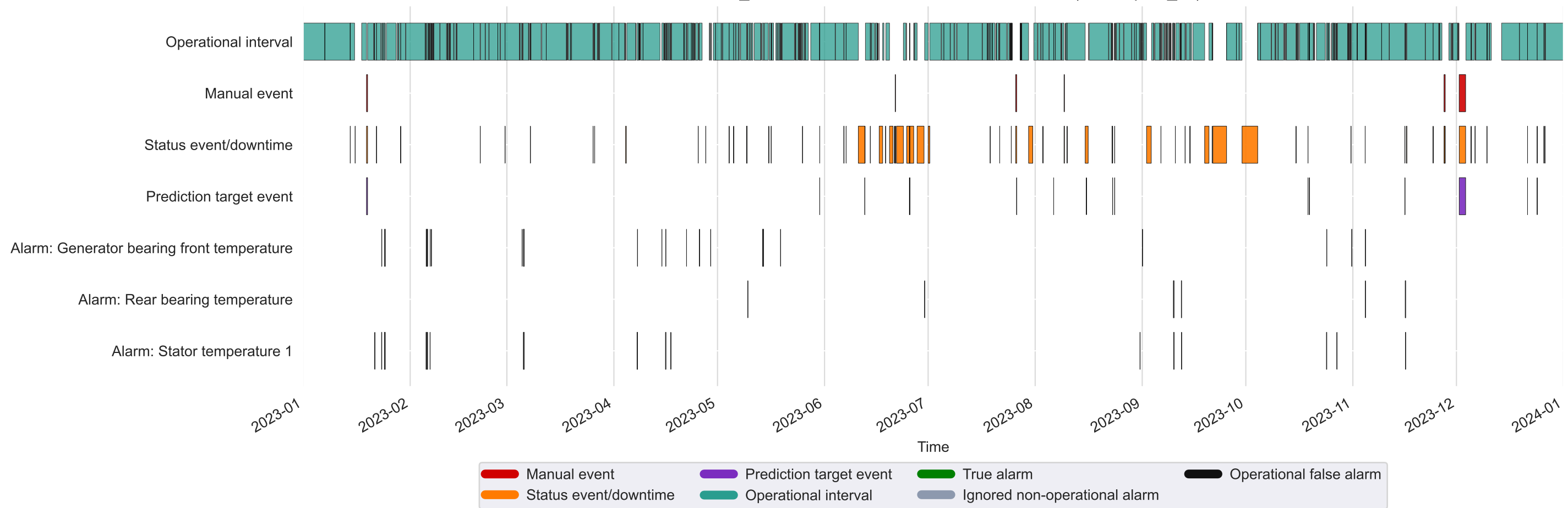
Kelmarsh_1: labelled intervals and detection alarms (2023, q995_c6)
