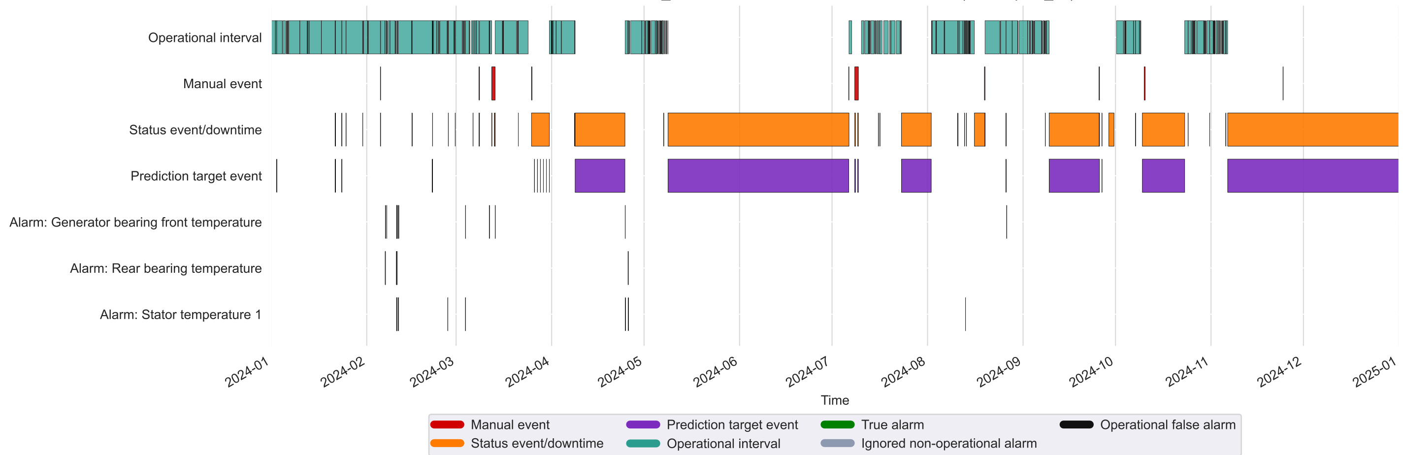
Kelmarsh_1: labelled intervals and detection alarms (2024, q995_c6)
