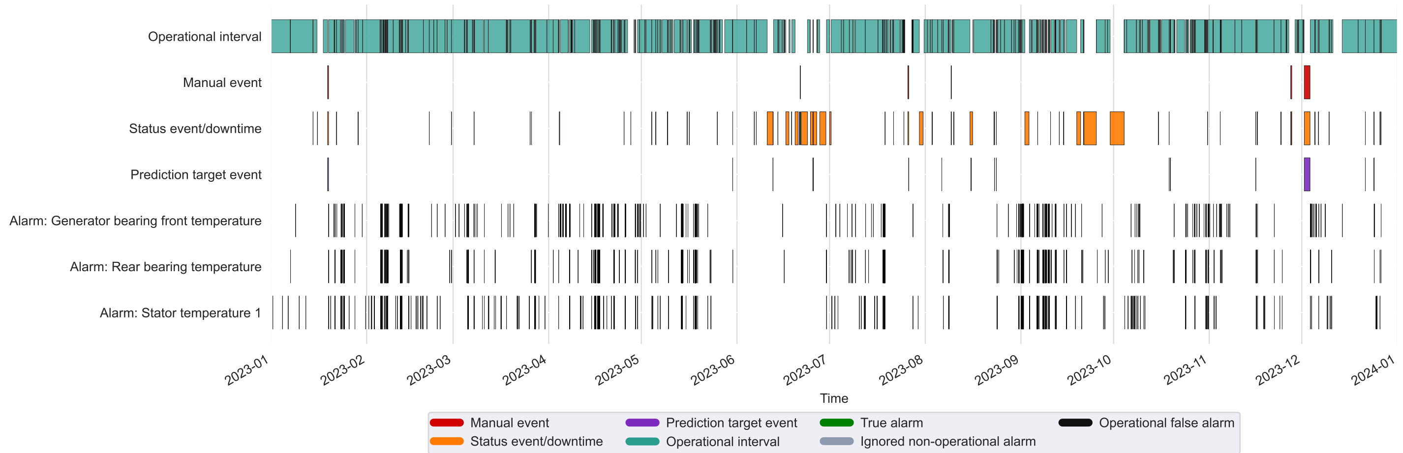
Kelmarsh_1: labelled intervals and detection alarms (2023, CUSUM, twosided_meanstd_k0p5_h5_c6_reset)
