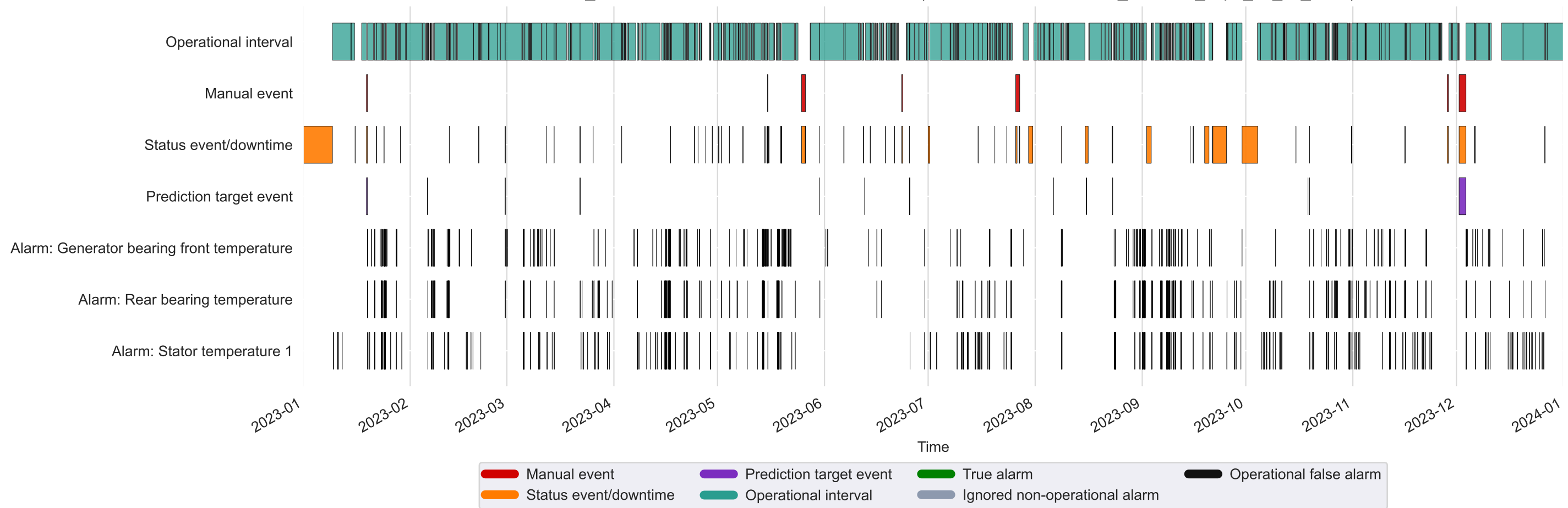
Kelmarsh_3: labelled intervals and detection alarms (2023, CUSUM, twosided_meanstd_k0p5_h5_c6_reset)
