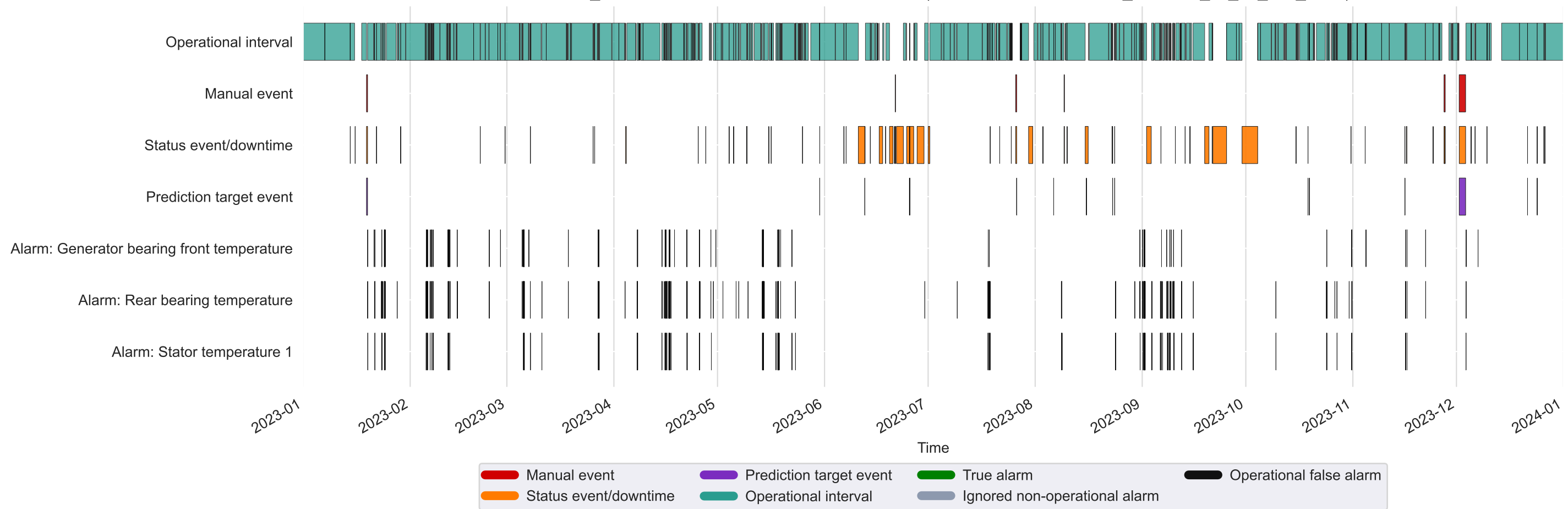
Kelmarsh_1: labelled intervals and detection alarms (2023, CUSUM, twosided_meanstd_k2_h5_c12_reset)
