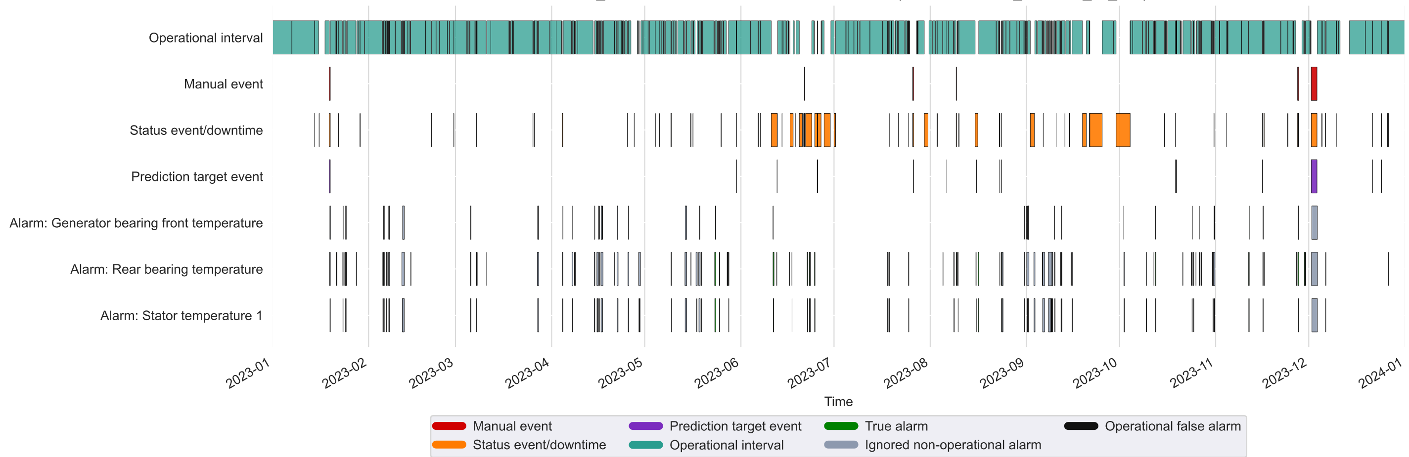
Kelmarsh_1: labelled intervals and detection alarms (2023, SCC, abs_meanstd_k3_c12)
