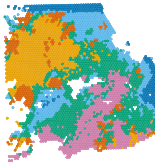
Spatial k-means
