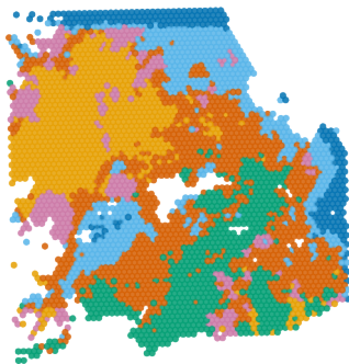
Expr-only k-means
