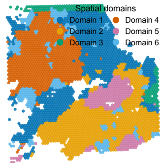
BayesSpace
