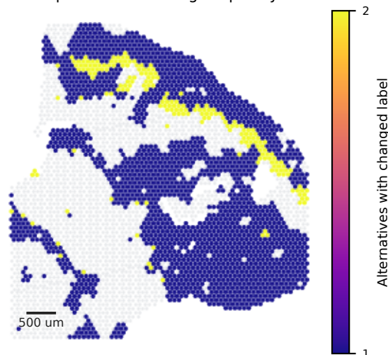
D TR11_206, BayesSpace, K=4 stable spots and switching frequency
