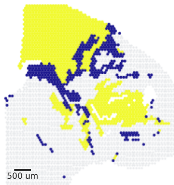
STAGATE-style
