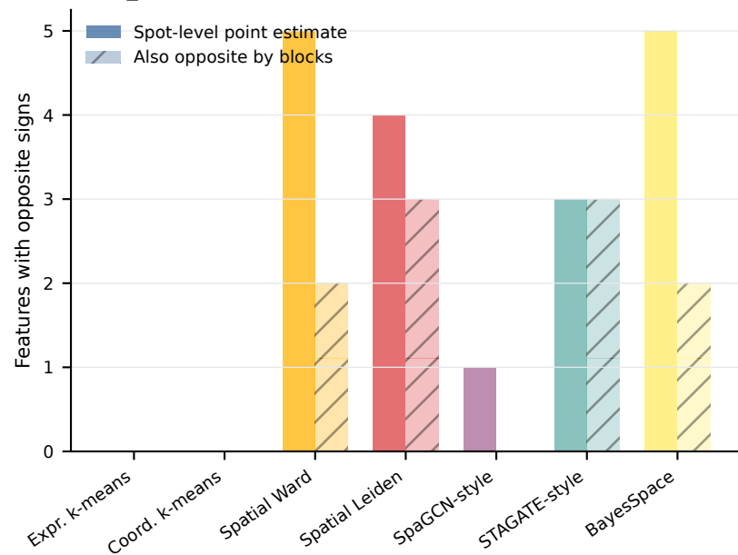
D TR11_206 across K=4 and K=6
