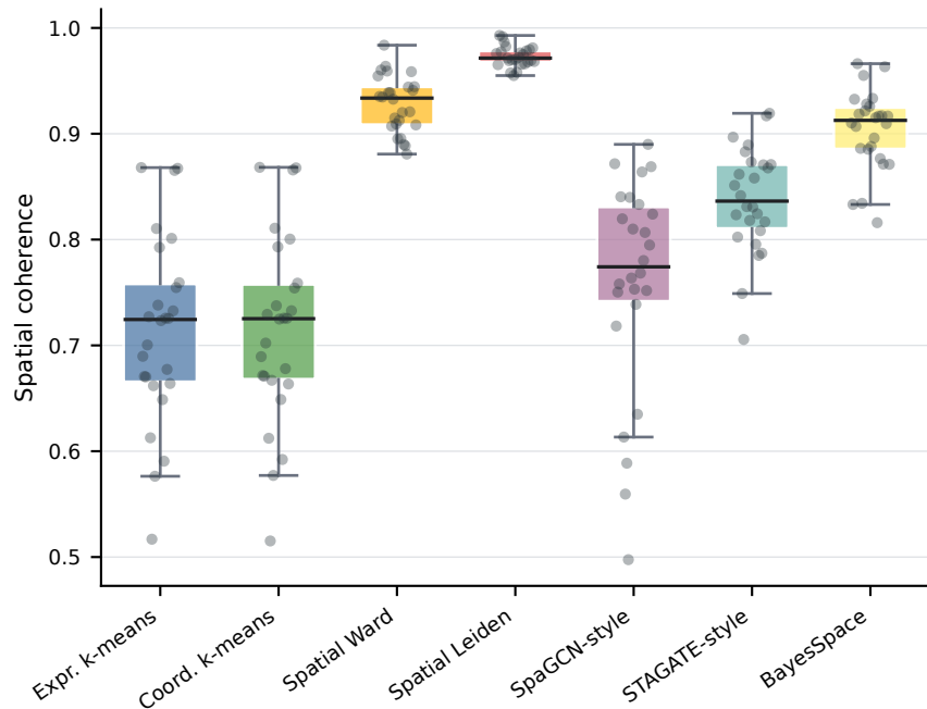
Spatial coherence across section-resolution settings
