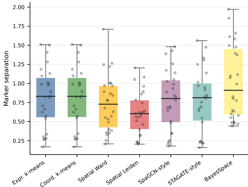
Marker separation across section-resolution settings
