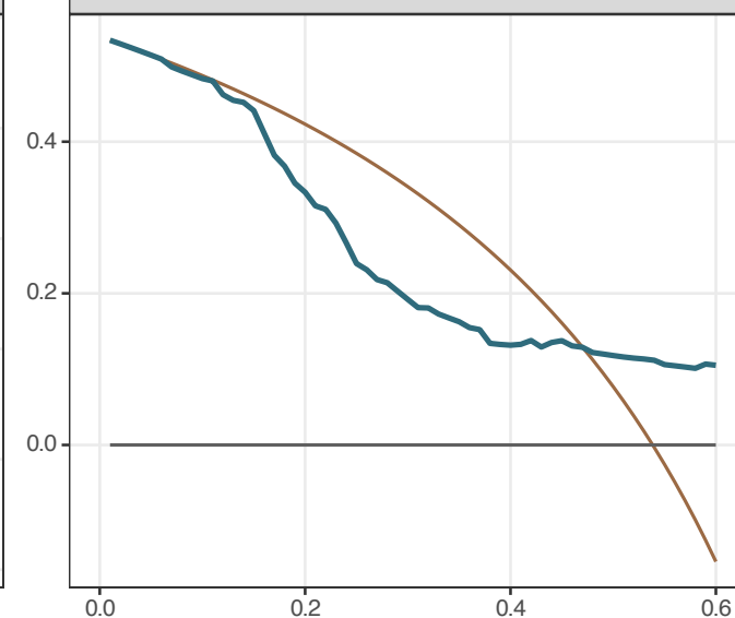
TCGA-LIHC
