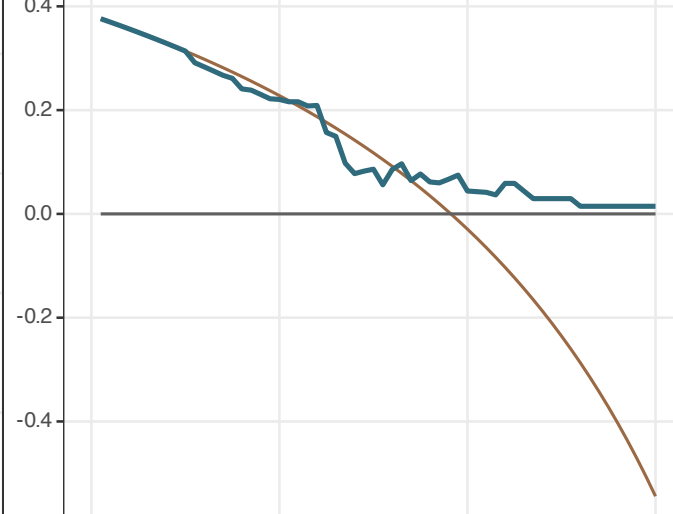
TCGA-LIHC
