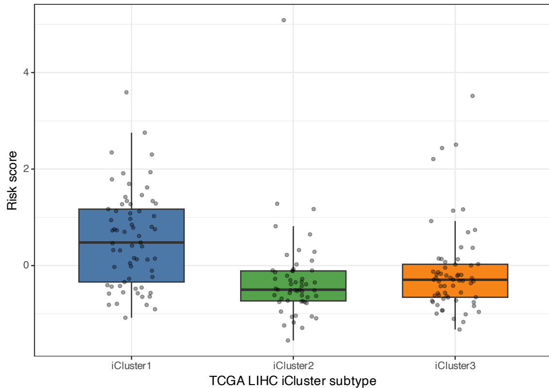
A Risk score by iCluster subtype (Kruskal P=1.9e-07)
