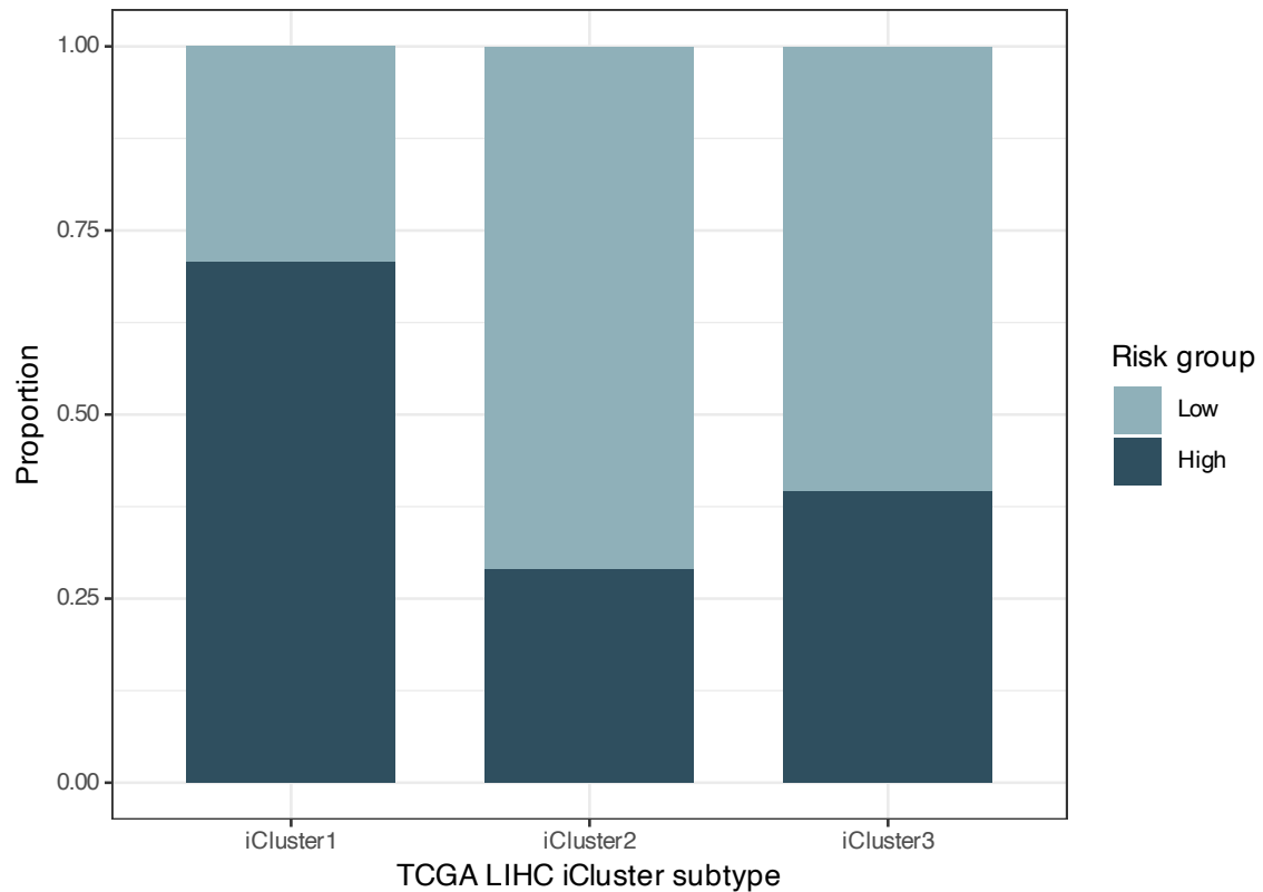
B Risk-group distribution by subtype (Chi-square P=9.5e-06)
