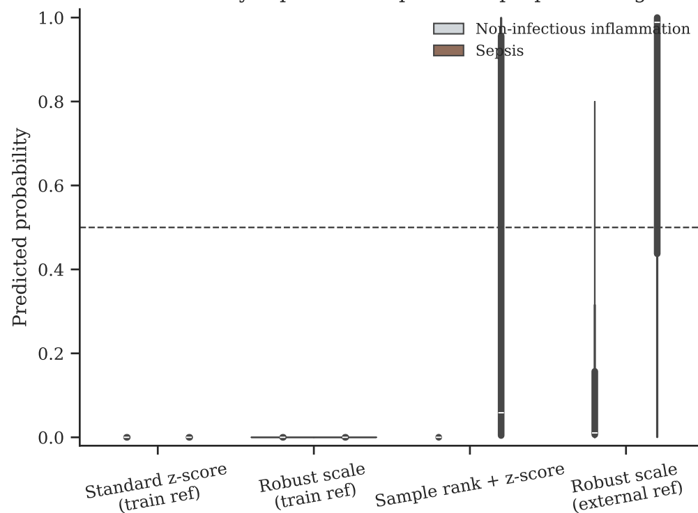
Probability separation depends on preprocessing
