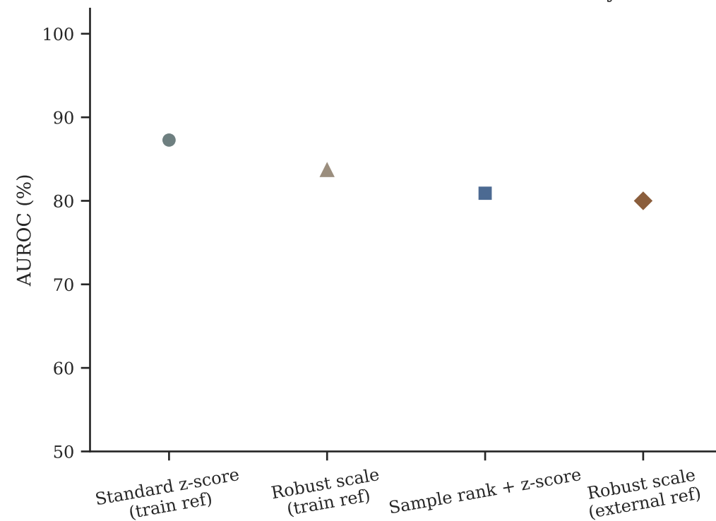
External AUROC alone overstates utility
