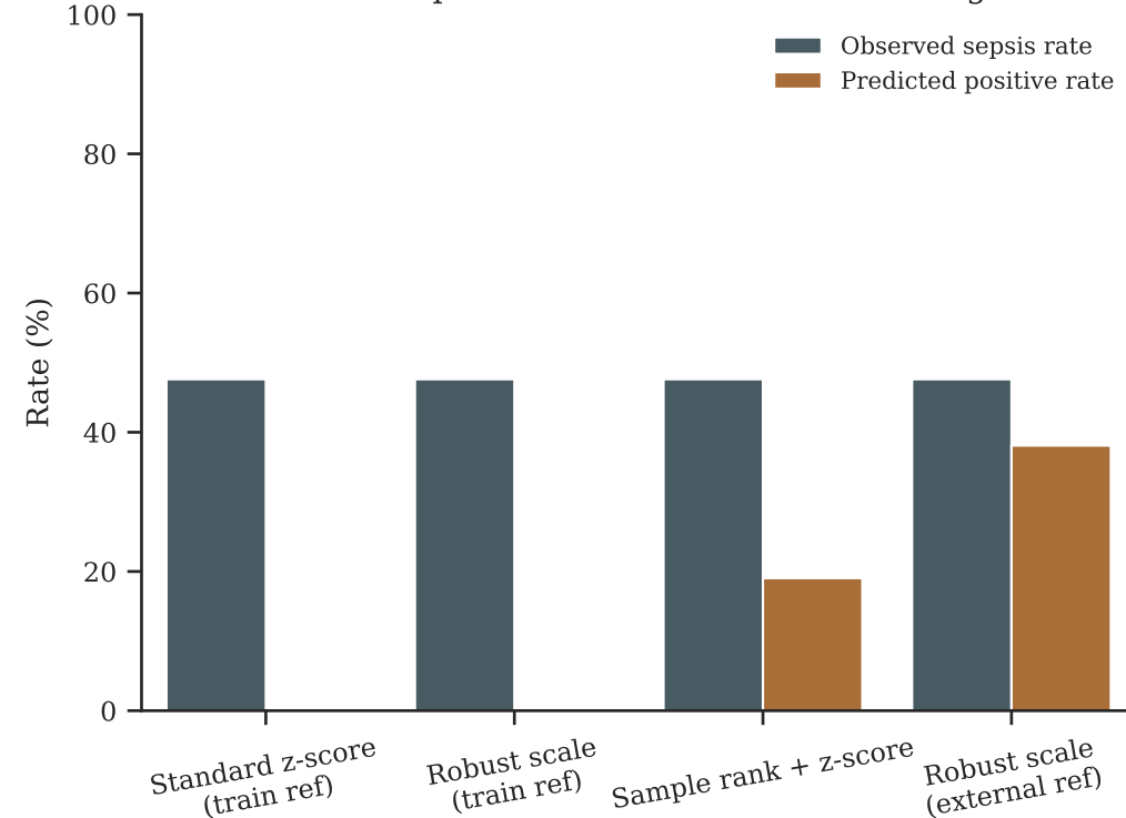
Observed and predicted rates under harder negatives
