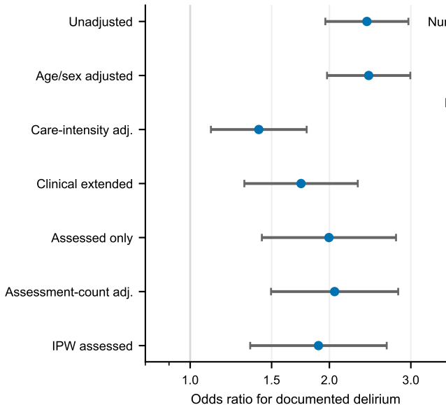
A Primary and ascertainment sensitivity models
