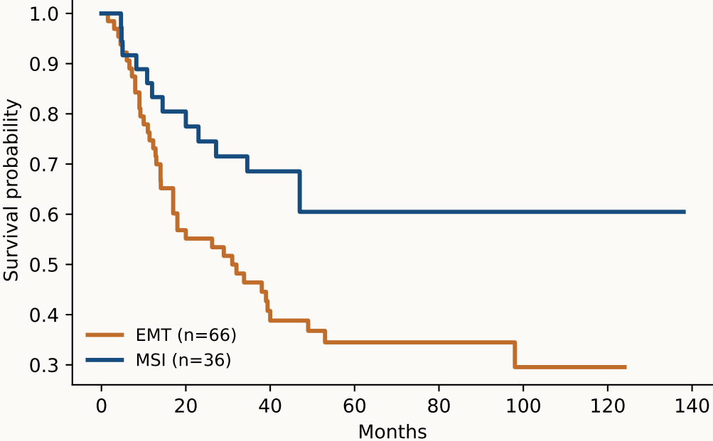
B GSE26942: overall survival (EMT vs MSI)
