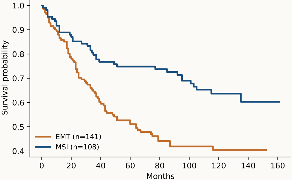
C GSE84437: overall survival (EMT vs MSI)
