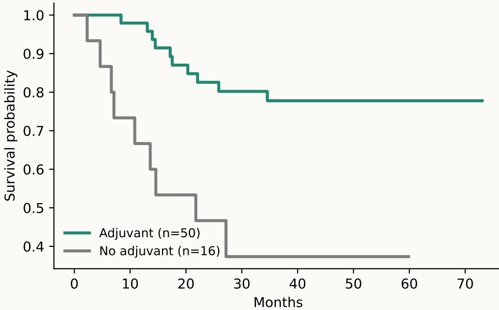
B GSE26899 (EP): adjuvant vs none
