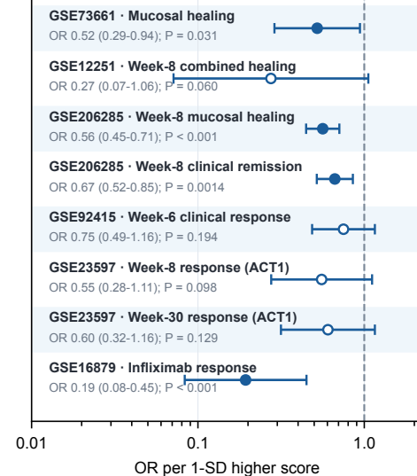
c GSE73661
