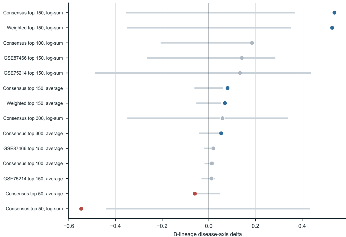
Figure S1. Disease-signature sensitivity
