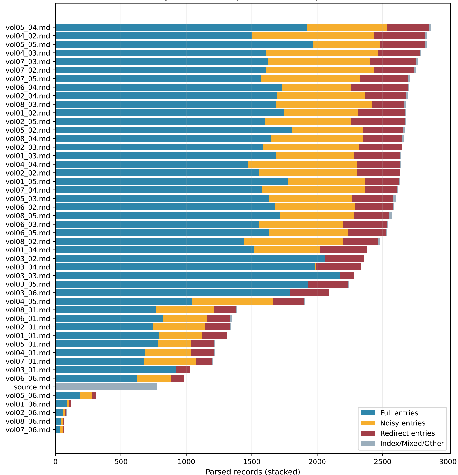
Figure 1. File-level parsed record composition
