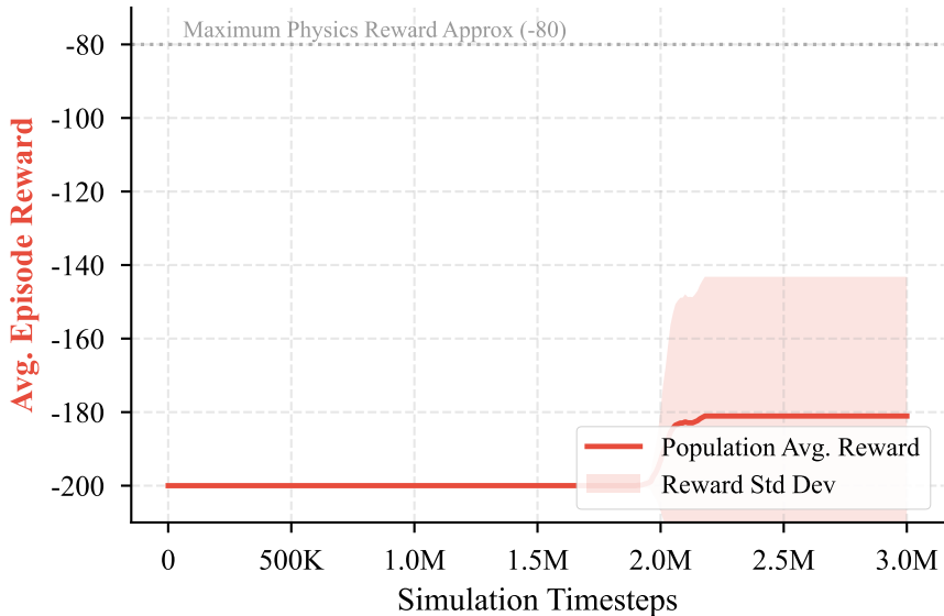
(b) PPO 3M Learning Curve (MountainCar Noisy)
