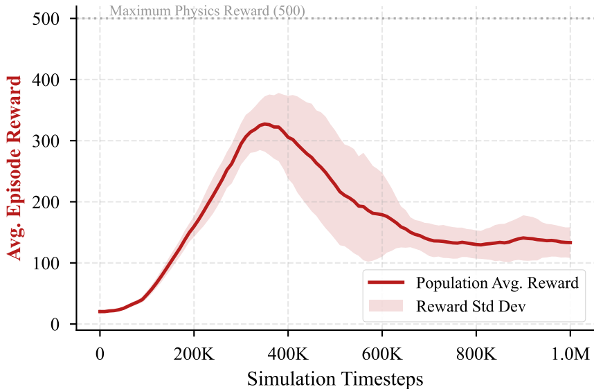
(b) PPO E2E Learning Curve (Noisy Environment)
