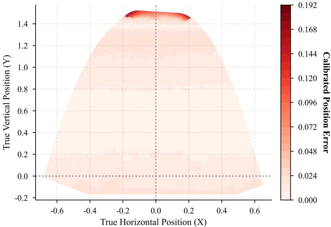
Calibrated Spatial Error Map (Free-fall Trajectories)
