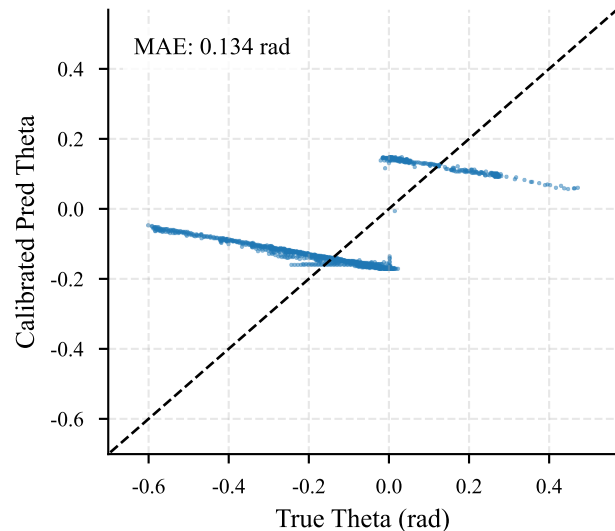
Orientation (Theta) Linearity
