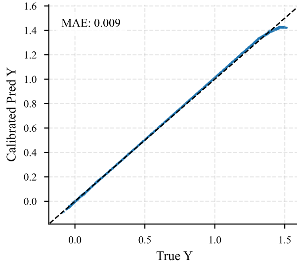
Vertical (Y) Linearity
