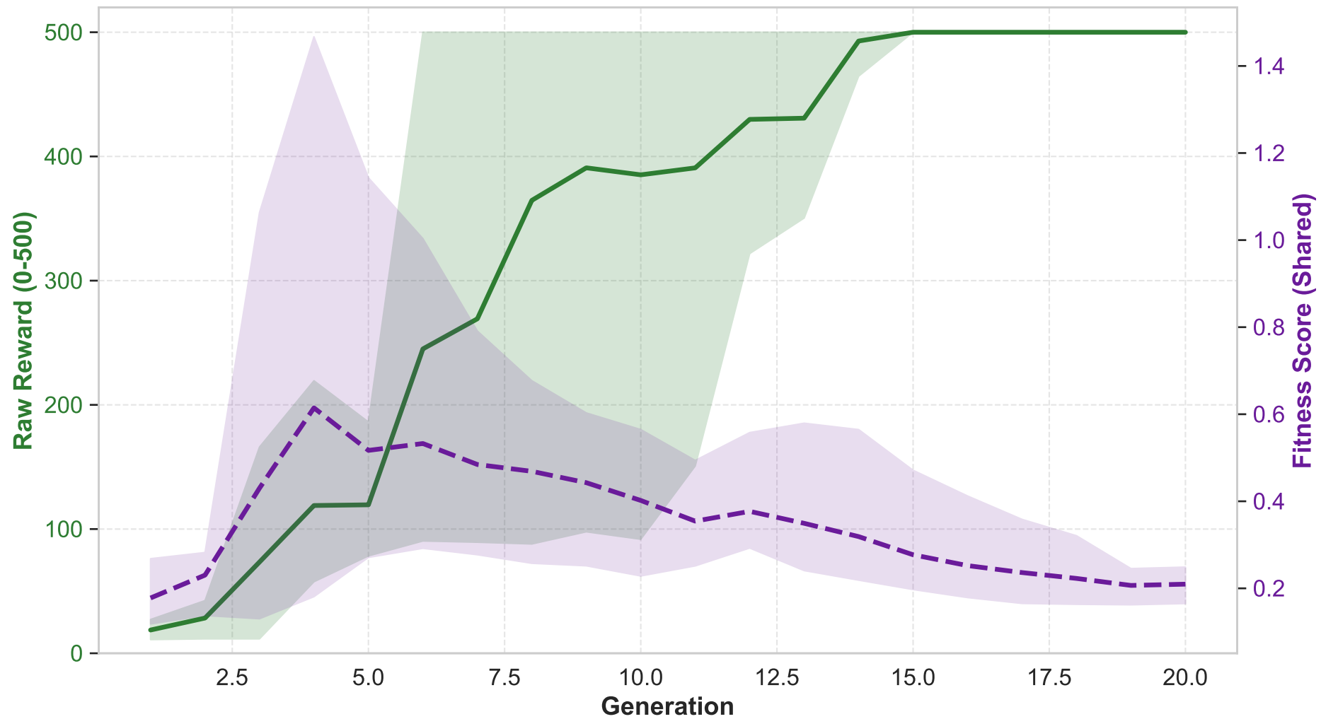
Training Dynamics: Reward vs. Fitness (N=5 Runs)
