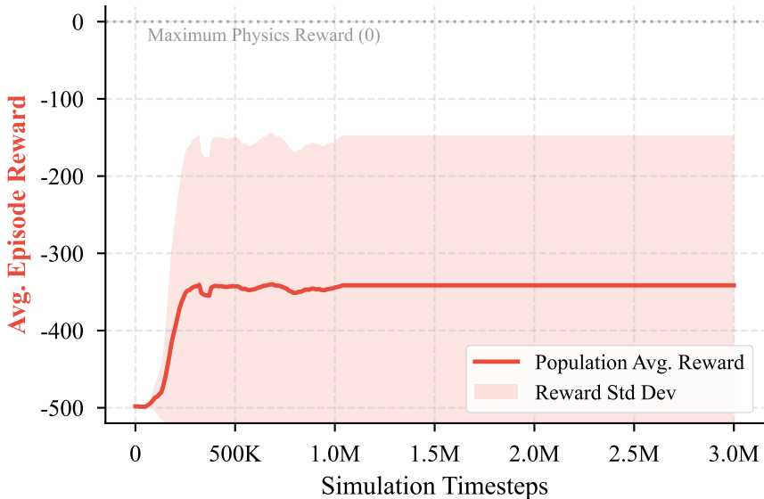
(b) PPO 3M Learning Curve (Acrobot Noisy)
