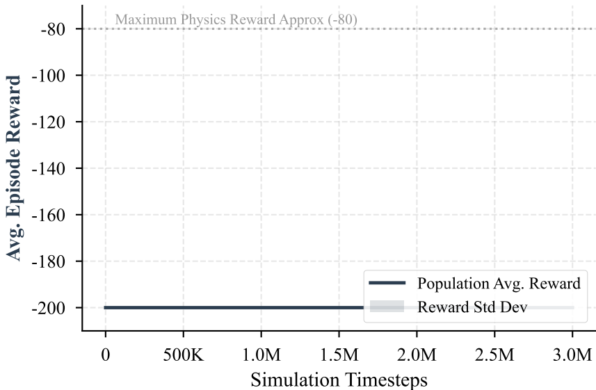
(a) PPO 3M Learning Curve (MountainCar Clean)
